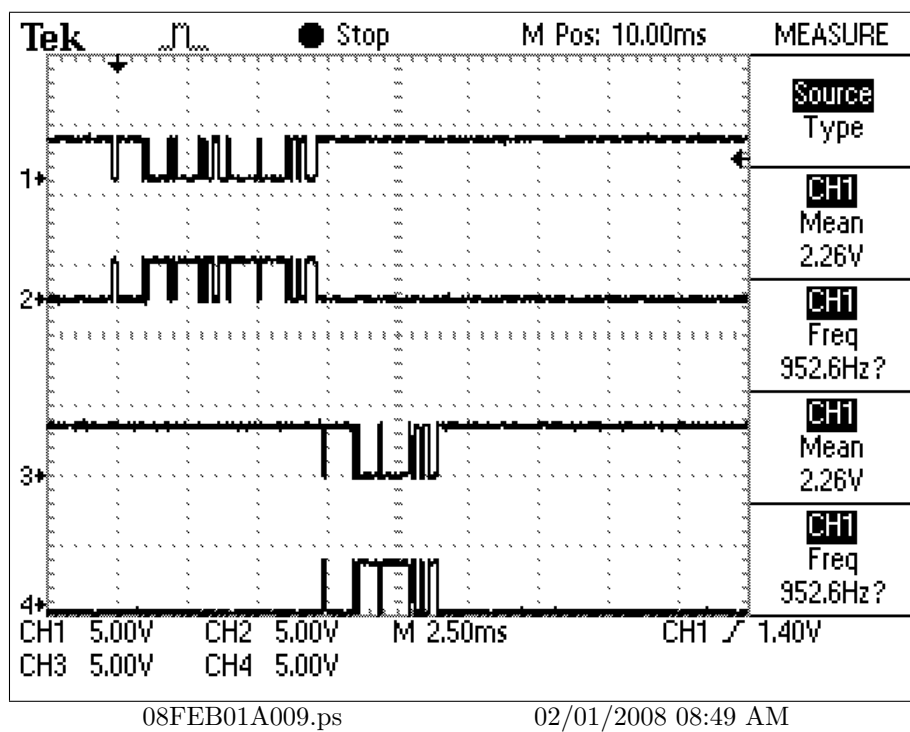
Figure 5: SW-2: 4,7,10 on, 5 off. Command and Reply.
