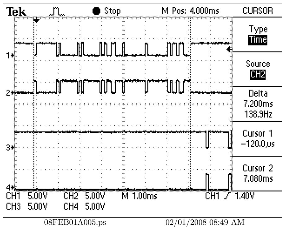
Figure 3: SW-2: 5,7,10 on, 4 off. Duration of the command.
