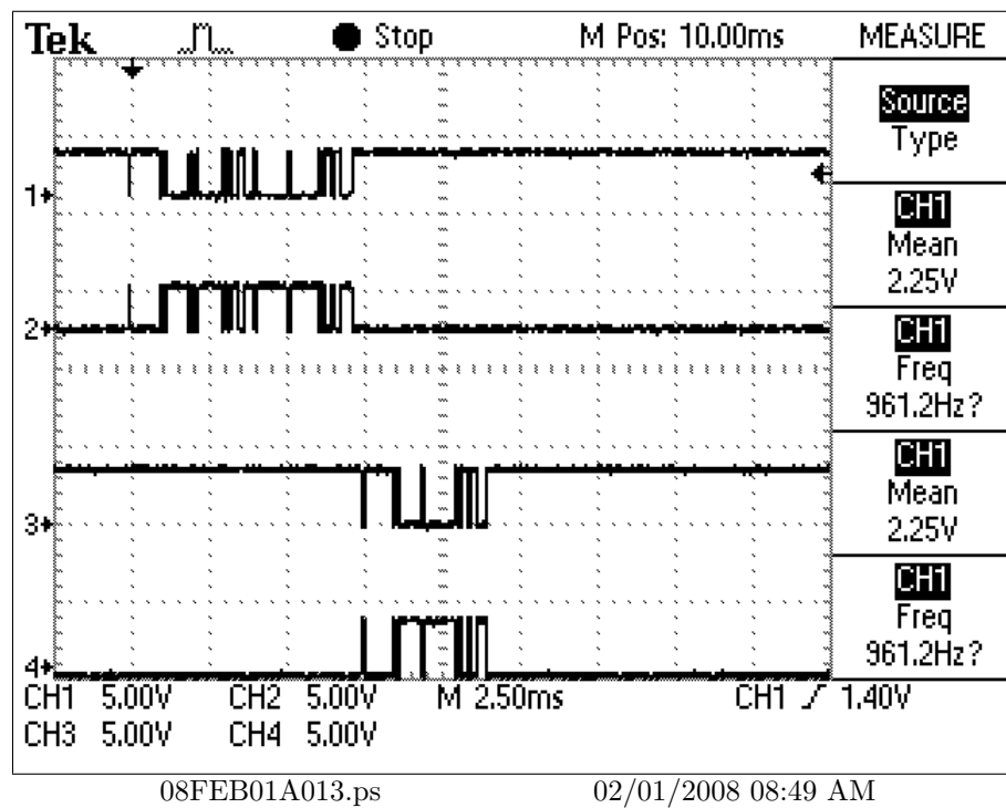
Figure 7: SW-2: 7,10 on, 4 & 5 off. Command and Reply.
