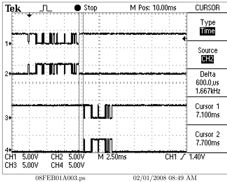
Figure 2: SW-2: 5,7,10 on, 4 off. Duration of the time between the end of a command and its reply. With full command and reply.
