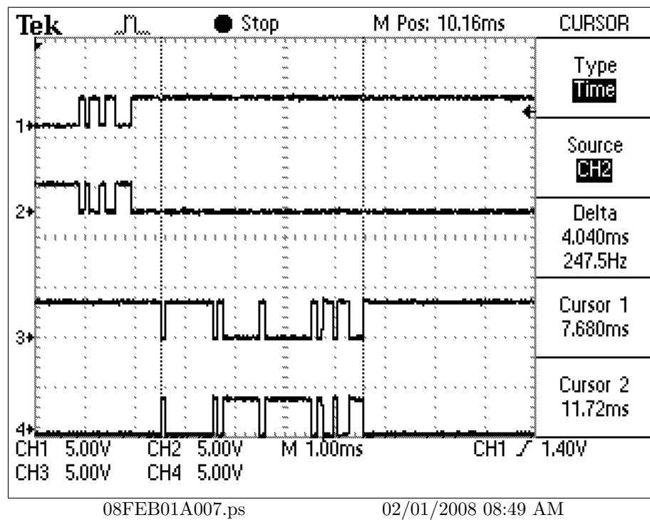
Figure 4: SW-2: 5,7,10 on, 4 off. Duration of the reply.
