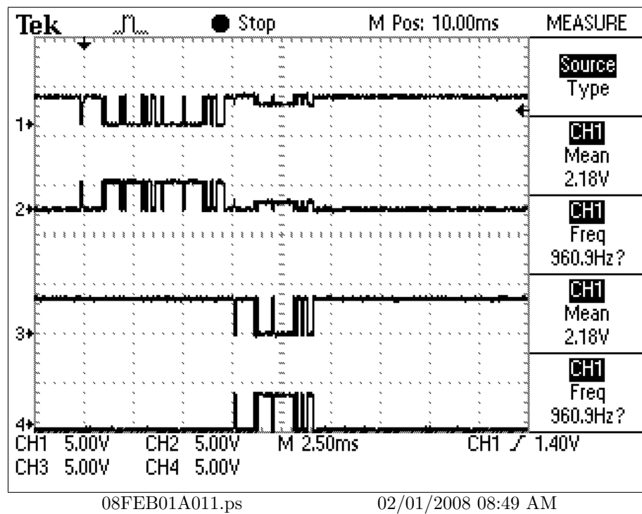
Figure 6: SW-2: 4,5,7,10 on. Command and Reply.
