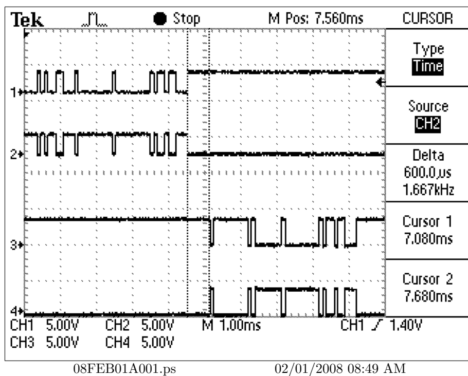
Figure 1: SW-2: 5,7,10 on, 4 off. Duration of the time between the end of a command and its reply. Expanded time.
