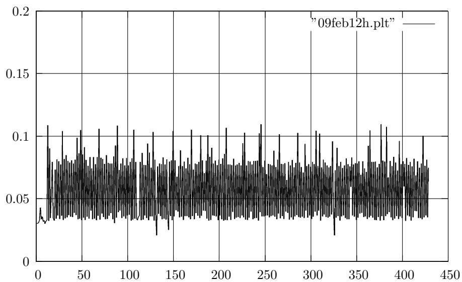
Figure 1: Plotted pan left/readout reply times from an Esprit ES31CBW24
