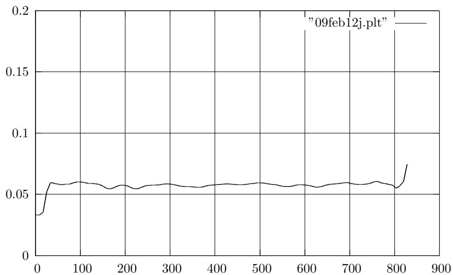
Figure 4: Plotted and smoothed pan left/tilt down/readout reply times from an Esprit ES31CBW24
