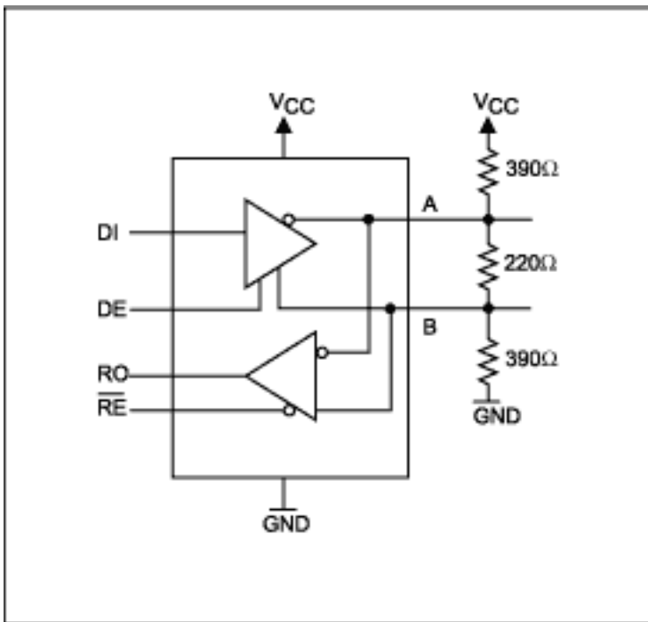
Figure 4. Typical RS-485 transceiver for PROFIBUS DP.
