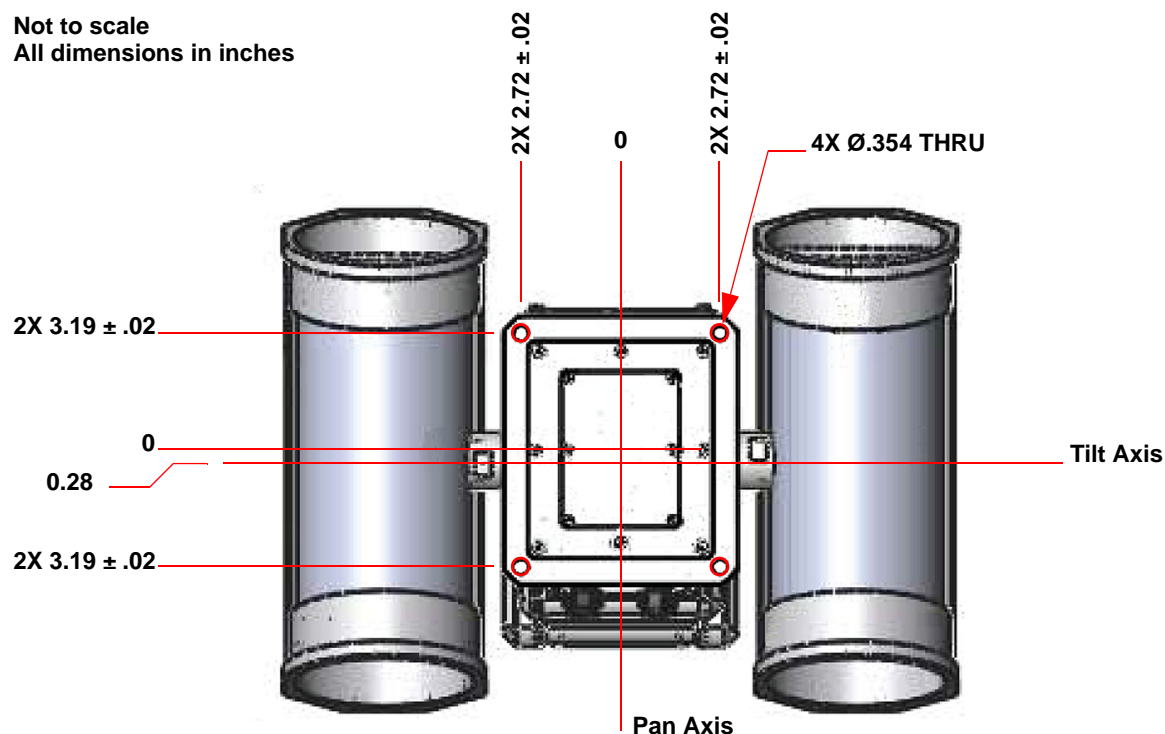
Figure 1-3: PT-Series Camera Mounting
