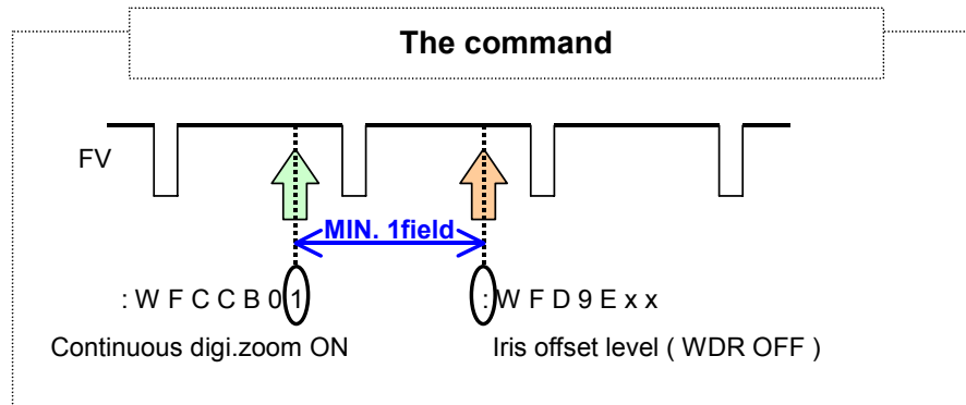
Fig. 2 Changed to command timing
