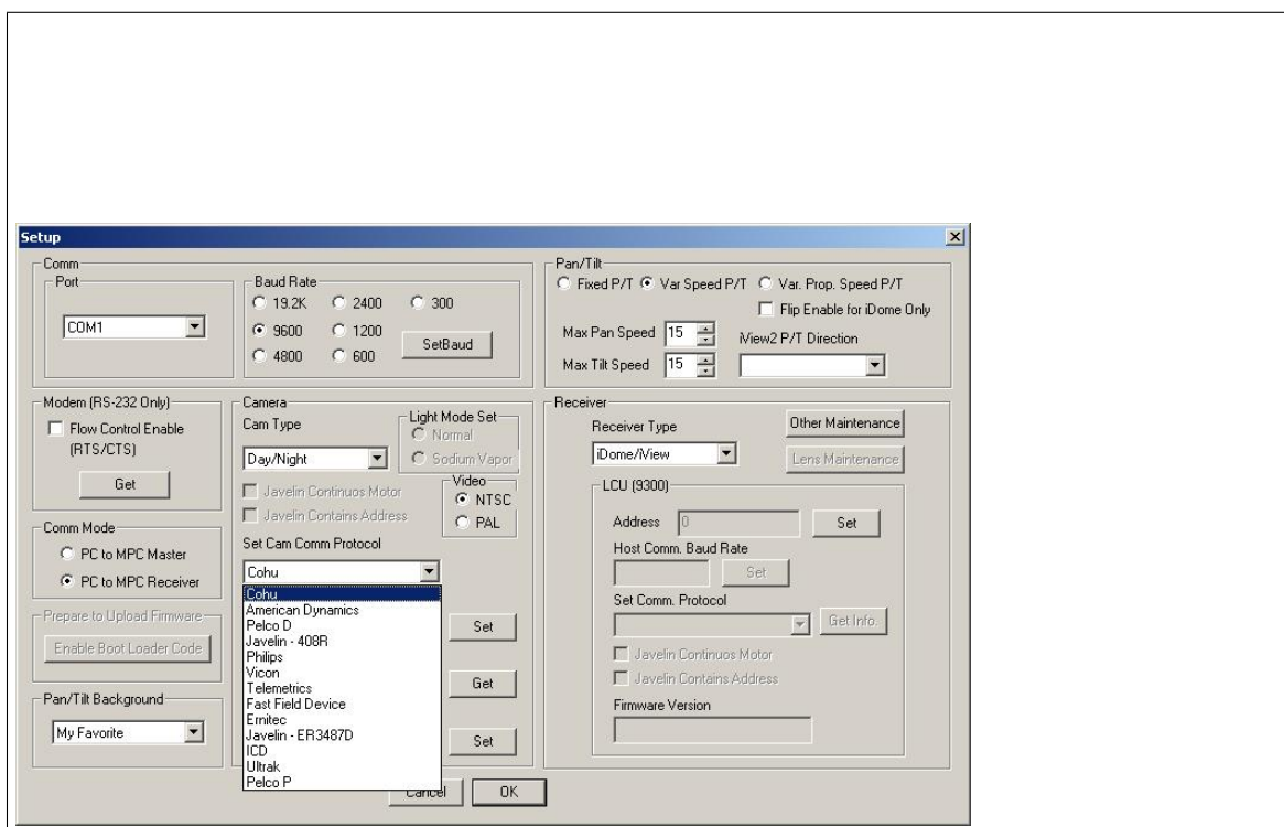
Figure 7: WinMPC, Camera Comm Protocol Window[xSetupSetCamCommProtocol.jpg]
