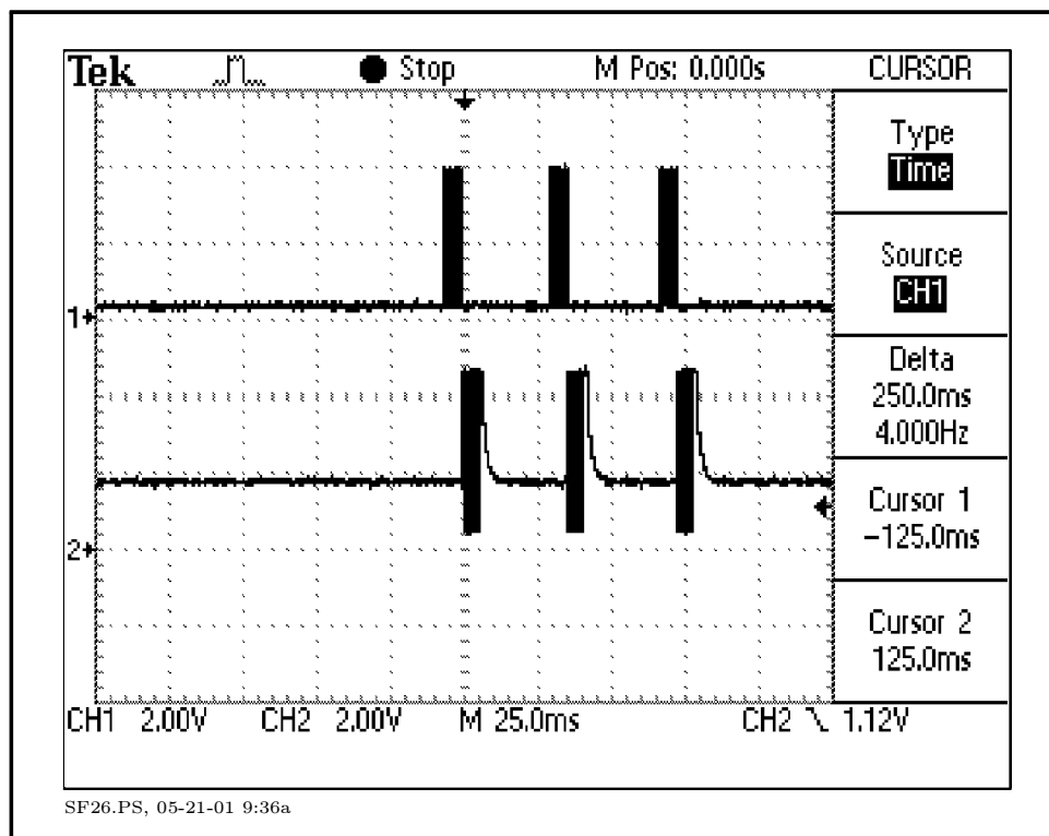
Figure 7. Fresno Sears, TXB-S422 Responses to “queries”.
