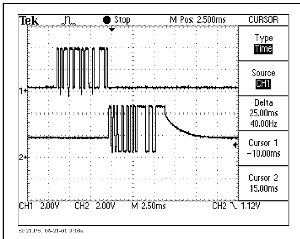
Figure 1. Fresno Sears, TXB-S422 First try
