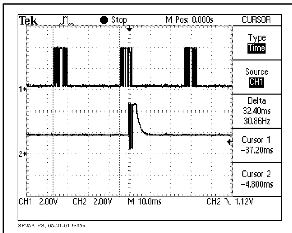
Figure 5. Fresno Sears, TXB-S422 Time between retransmitted commands.
