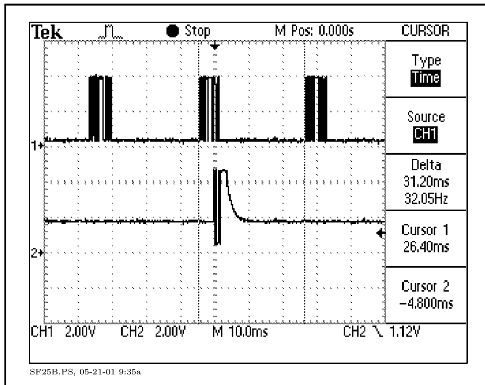
Figure 6. Fresno Sears, TXB-S422 Second time between retransmitted commands.
