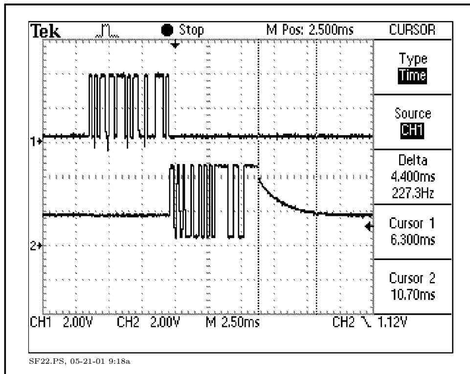
Figure 2. Fresno Sears, TXB-S422 Duration of the return to quiescent.
