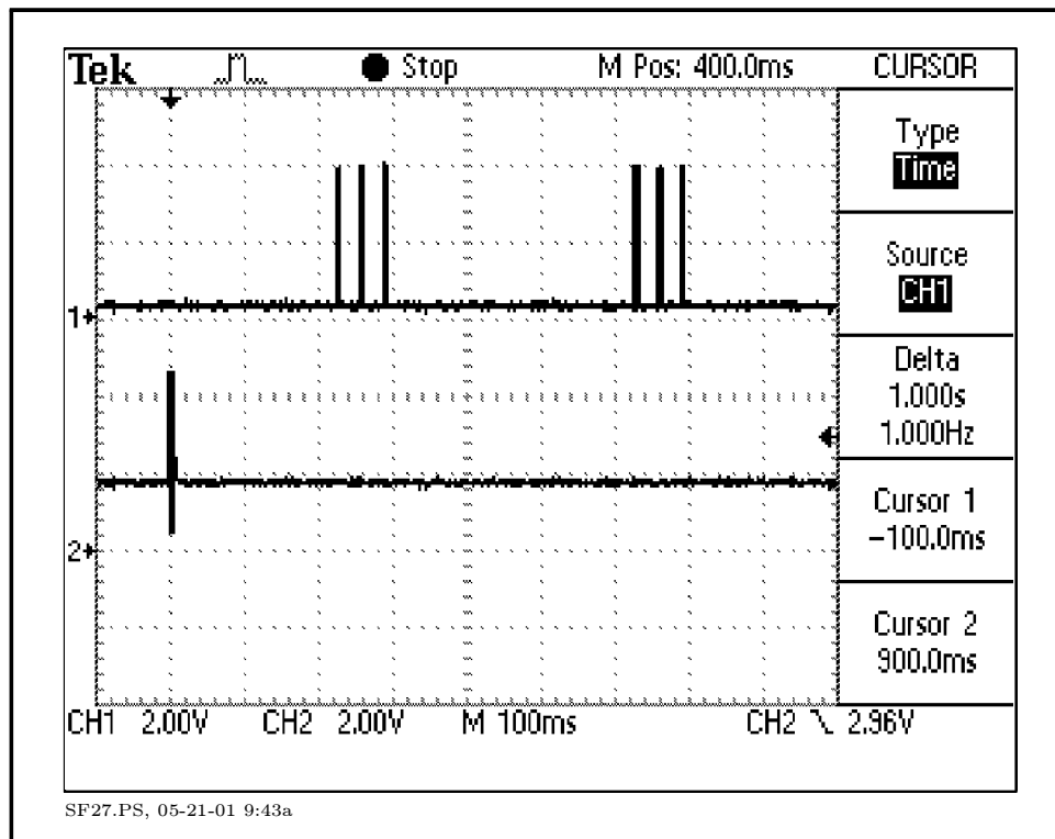
Figure 8: Fresno Sears, TXB-S422 Power up sequence. Note that the controller's response is missing.
