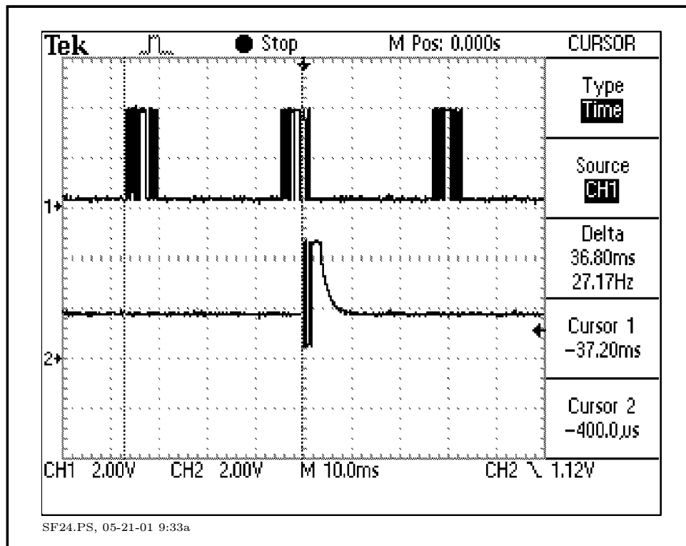
Figure 4. Fresno Sears, TXB-S422 Time from start of a command to its reply.
