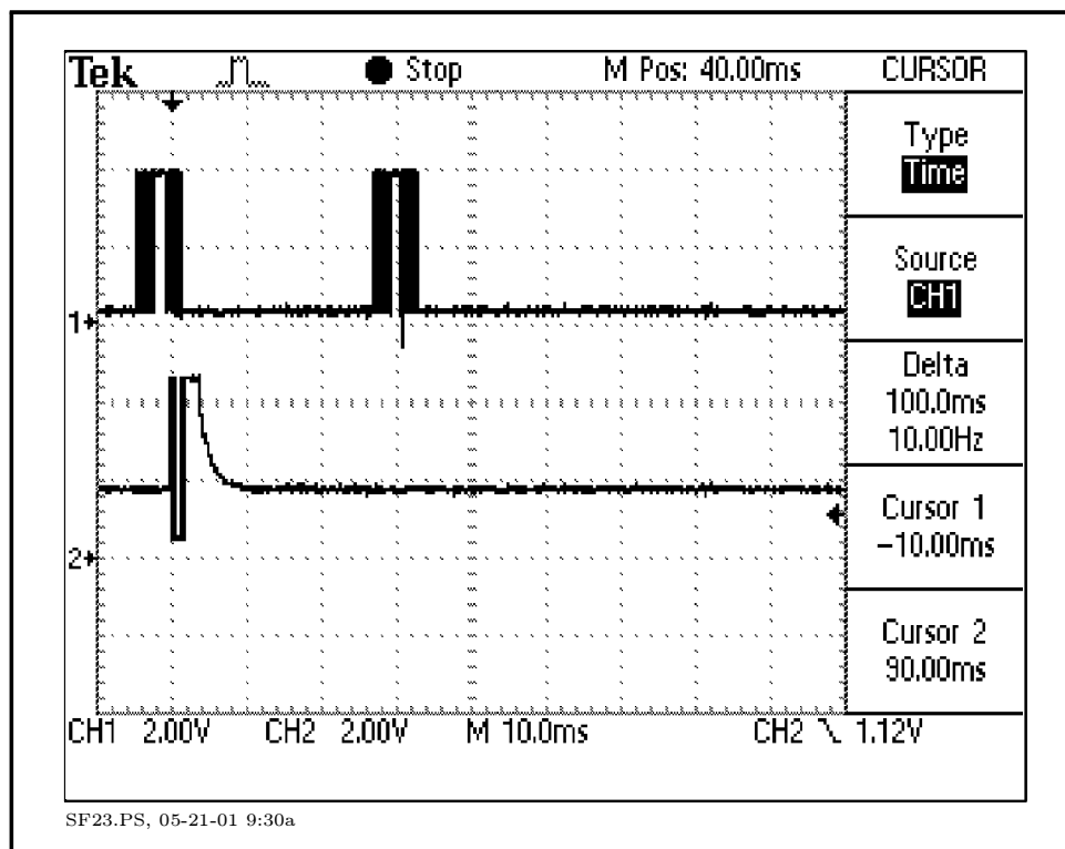
Figure 3. Fresno Sears, TXB-S422 Reply to a command.
