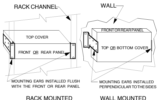
Figure 2 - Mounting Options
