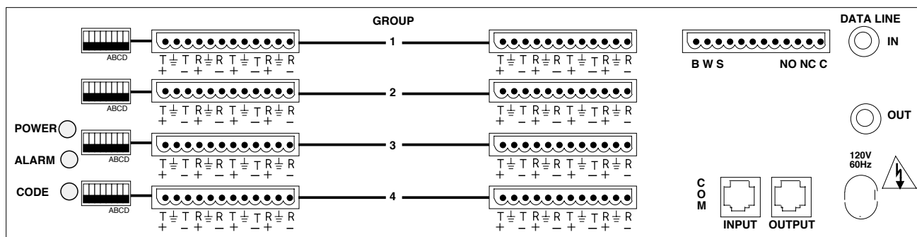
Figure 1-2083-02B Code Translator Rear Panel
