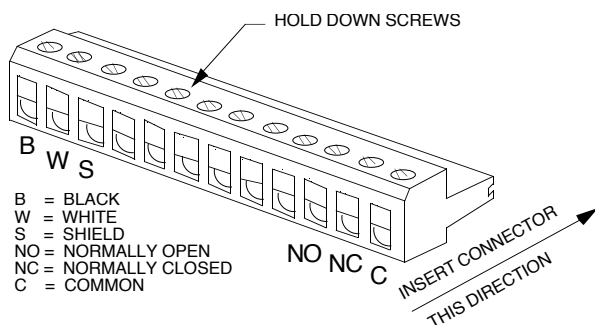
Figure 5 - Control Code Mating Connector
