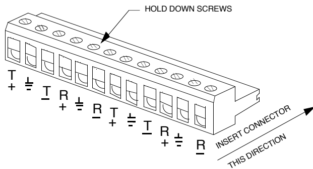
Figure 4 - Typical Mating Screw Connector
